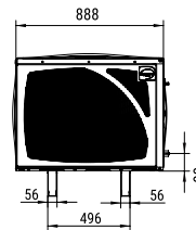
FRONTAL VIEW VISTA FRONTAL
