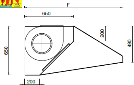
Modelo Pared Vent 400°/2h
